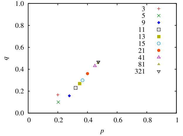
Fig. 5: (Colour on-line) The average of victorious (p, q) values, as obtained for different values of N > 5 . For comparison, we also plot the average of surviving strategies for N = 3 and N = 5 , where stable coexistence can be observed. The trace of destinations shows clearly that the final average (p, q) values converge to the fair p = q \approx 0.5 solution as we increase N .
