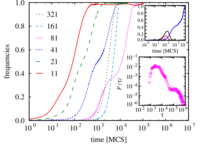
Fig. 3: (Colour on-line) Time evolution of the fraction of the single surviving strategy for different values of N > 5 (see legend) and L=800 . The upper inset shows the time evolution of the three strategies competing the longest, as obtained for N=41 and L=400 . As an illustration of how the fixation time fluctuates, the lower inset shows the probability distribution of the fixation time \tau , as obtained for N=81 and L=200 , and averaged over 10^4 independent realizations of the game.
