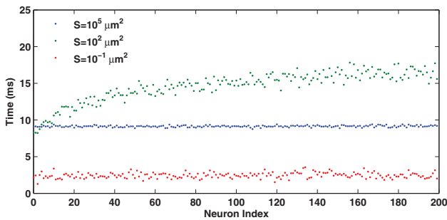
Fig. 1: (Colour on-line) Spatiotemporal distribution of first spikes produced by 200 scale-free-coupled Hodgkin-Huxley neurons driven by a supra-threshold periodic stimulus f(t) with frequency \nu = 20 Hz and amplitude A = 4 \mu\text{A}/\text{cm}^2 for different membrane areas S , as indicated in the figure legend. An intermediate intensity of internal noise at S = 100 \mu\text{m}^2 induces maximal delays, which however are less pronounced by high-degree neurons (low neuron index i ) than by low-degree neurons. This hints towards the fact that the heterogeneity of the interaction network might play a key role in mitigating prolonged first-spike latency. The employed coupling strength is \varepsilon = 0.01 .
