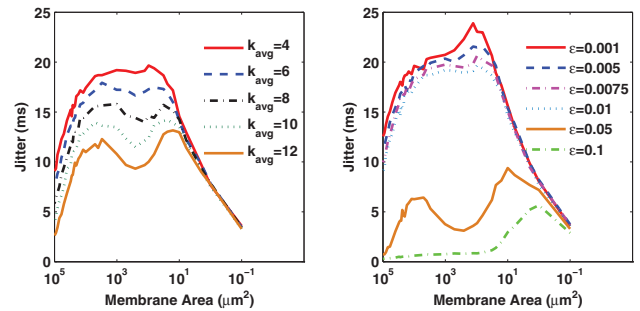
Fig. 6: (Colour on-line) Temporal jitter in dependence on the membrane area S , as obtained for different average degrees k_{avg} (left) and coupling strengths \varepsilon (right) in the presence of sodium channel blocking ( x_{Na} = 0.95 and x_K = 1 ). Here too the coupling strength plays a key role in reducing the signature of noise-delayed decay, while the impact of average degree is much more subtle. The increase of both \varepsilon and k_{avg} , however, introduces a peculiar double-peak structure in dependence on S , which indicates competition between local and global effects affecting the delayed responsiveness of the neuronal network.
