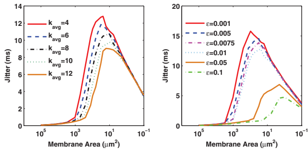
Fig. 5: (Colour on-line) Temporal jitter in dependence on the membrane area S , as obtained for different average degrees k_{avg} (left) and coupling strengths \varepsilon (right) in the presence of potassium channel blocking ( x_K = 0.95 and x_{Na} = 1 ). Similarly as concluded from results presented in figs. 2 and 3, in case of potassium channel blocking too the coupling strength plays a much more significant role than the average degree in ensuring high responsiveness of the neuronal network.
