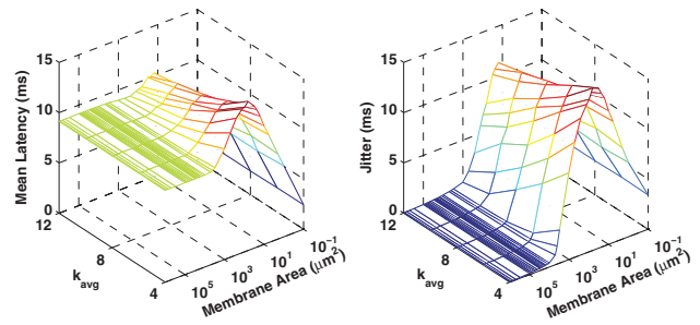
Fig. 2: (Colour on-line) Mean latency \Lambda (left) and jitter \Psi (right) in dependence on the average degree k_{avg} and the membrane area S , as obtained for \nu = 20 Hz, A = 4 \mu\text{A}/\text{cm}^2 and \varepsilon = 0.01 . It can be observed that there exists an intermediate internal noise intensity at which both \Lambda and \Psi are maximal. Although the peak values decrease with increasing k_{avg} and also shift towards slightly larger values of S , the relevance of the average degree of individual neurons is fairly marginal.
