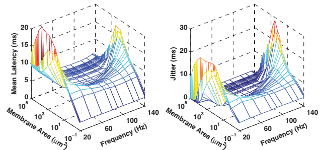
Fig. 4: (Colour on-line) Mean latency \Lambda (left) and jitter \Psi (right) in dependence on the frequency of the external signal and the membrane area S , as obtained for \varepsilon = 0.01 , k_{avg} = 4 and A = 4 \mu\text{A}/\text{cm}^2 . It can be observed that low and high frequencies are significantly more elusive to detection than intermediate frequencies of the external signal. The latter yield a clear decrease in both \Lambda and \Psi , although an intermediate values of S still proves to be the most damaging to early detection. These results are largely robust to variations of \varepsilon and k_{avg} , and they also agree with preceding observations made on individual neurons.
