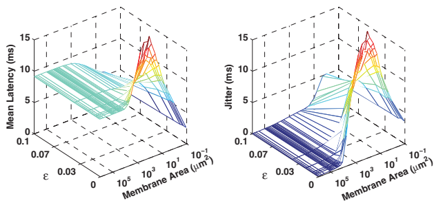
Fig. 3: (Colour on-line) Mean latency \Lambda (left) and jitter \Psi (right) in dependence on the coupling strength \varepsilon and the membrane area S , as obtained for \nu = 20 Hz, A = 4 \mu\text{A}/\text{cm}^2 and k_{avg} = 4 . As in fig. 2, it can be observed that there exists an intermediate internal noise intensity at which both \Lambda and \Psi are maximal. As \varepsilon increases, however, the peak values decrease significantly, and at sufficiently strong coupling the signature of noise-delayed decay appears to altogether vanish. This indicates that the coupling strength plays a more pivotal role than average degree in mitigating delayed first-spike onset in neuronal networks.
